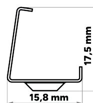
BARDE+ METAL MOUNTING CLIP / UCHWYT
