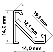
BARDE+ ALUMINIUM LED PROFILE / PROFIL LED
