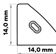
BARDE+ PLASTIC END CAP / ZAŚLEPKA
